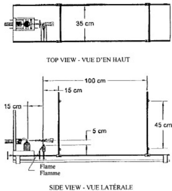
FIGURE 2 Flammability Tester Pump-Spray Container
