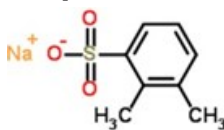
Figure 31. Sodium dimethylbenzene sulphonate
