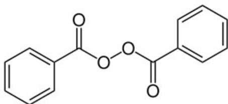
Figure 24. Benzoyl peroxide
