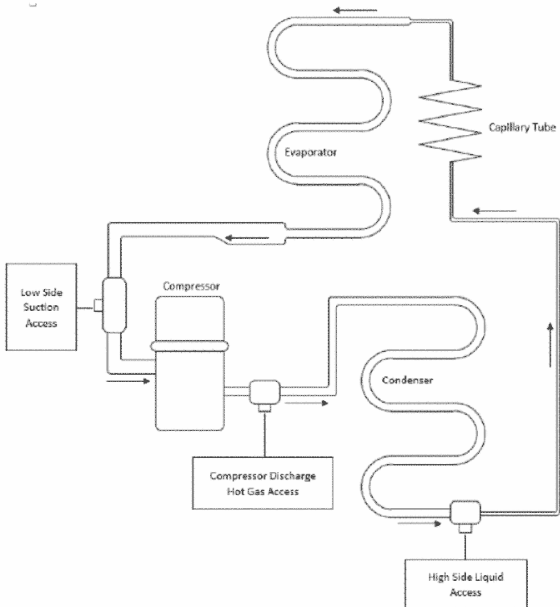
Figure 2. System Dependent Equipment Test Apparatus
