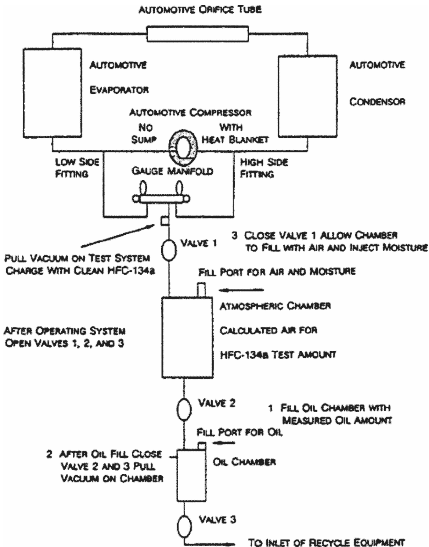
FIGURE 1 - TEST FIXTURE
