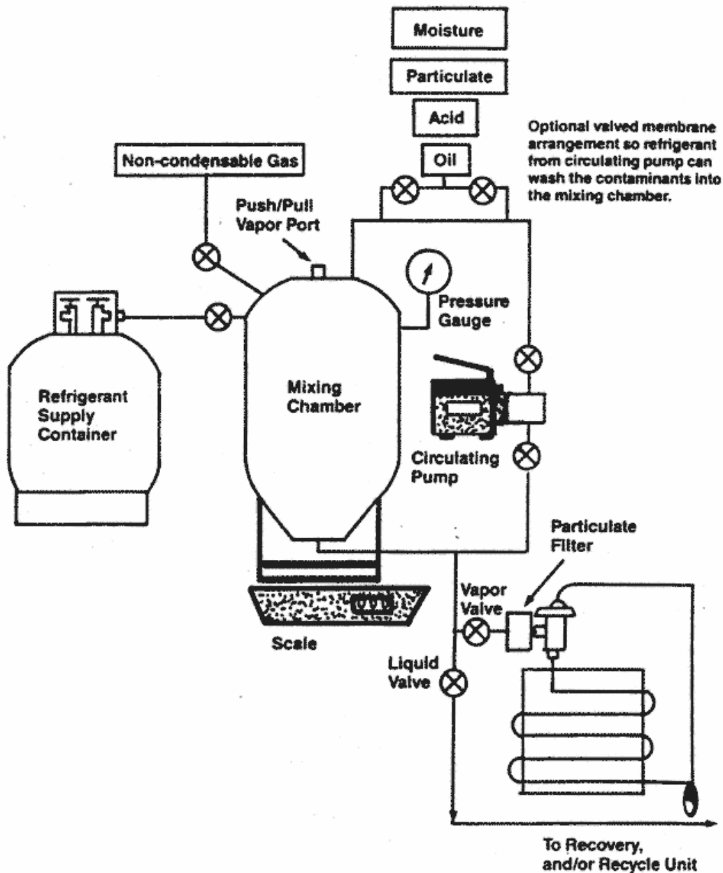
Figure 1. Test Apparatus for Self-Contained Equipment
