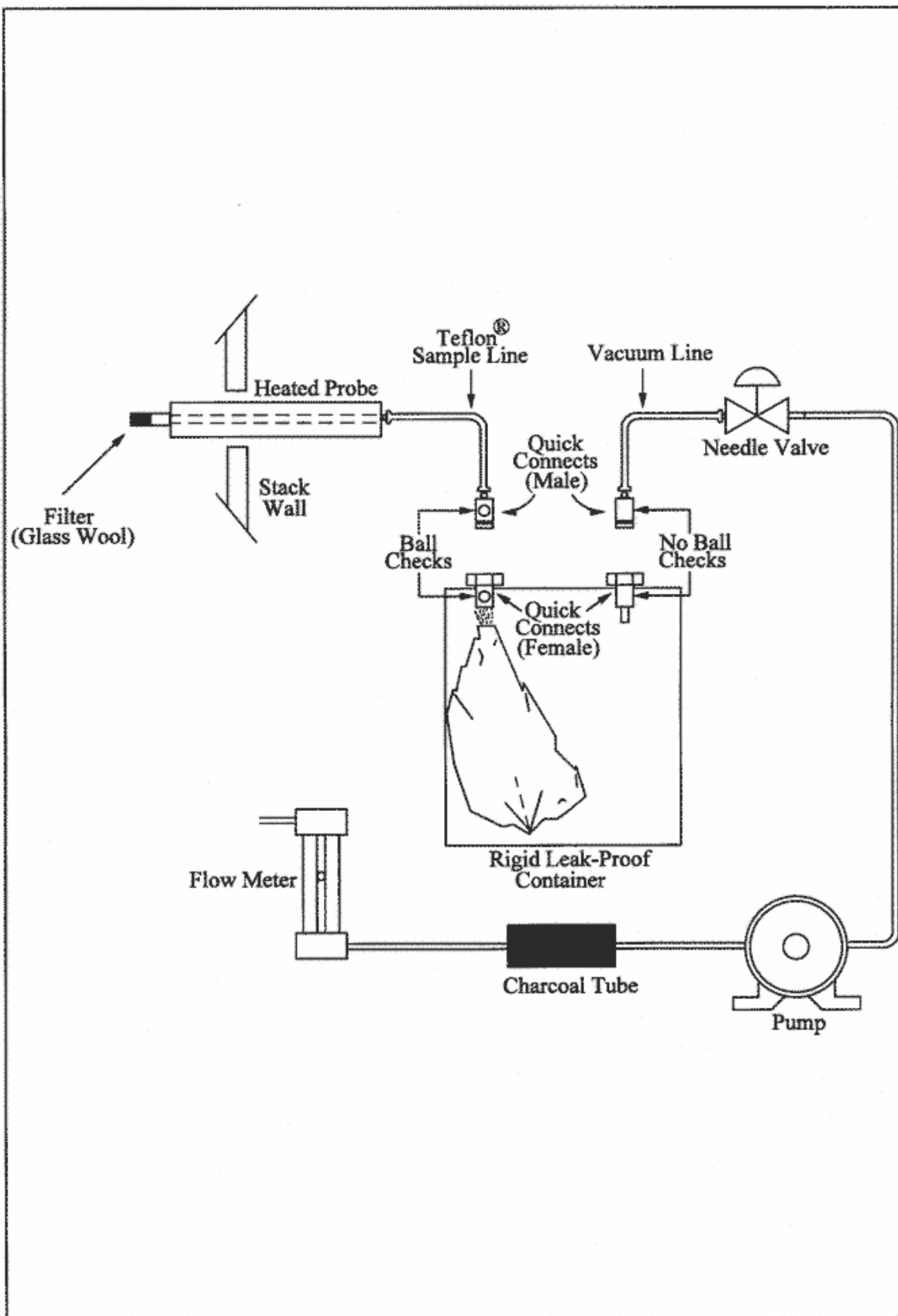
Figure 106-1. Integrated-bag sampling train.
