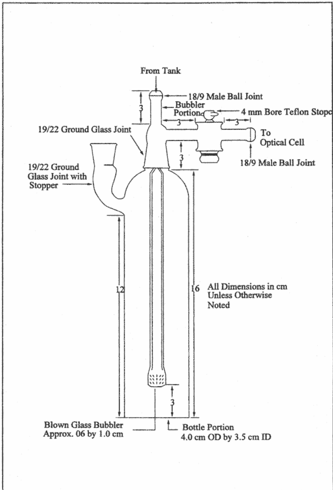
Figure 101-3. Aeration Cell.
