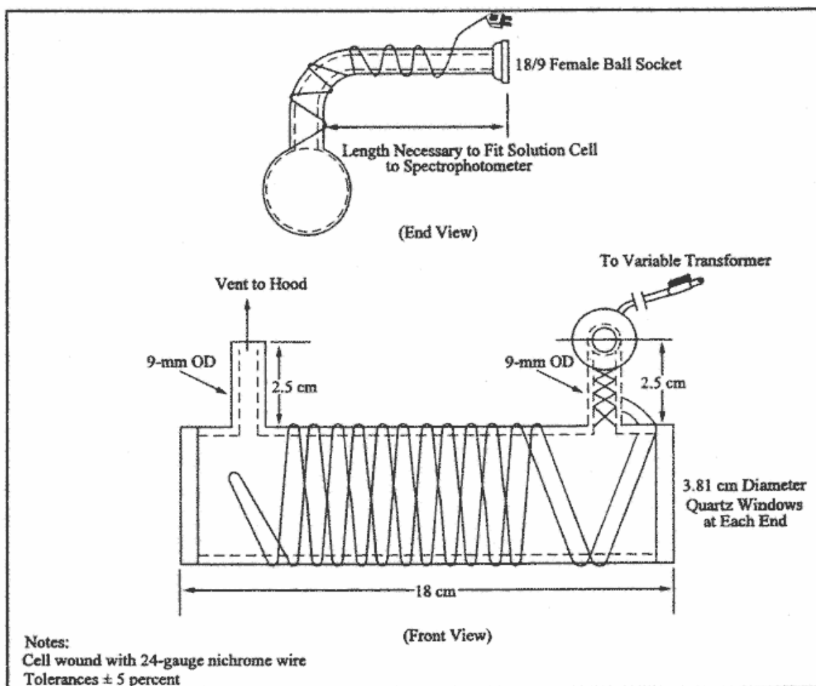
Figure 101-2. Optical Cell.
