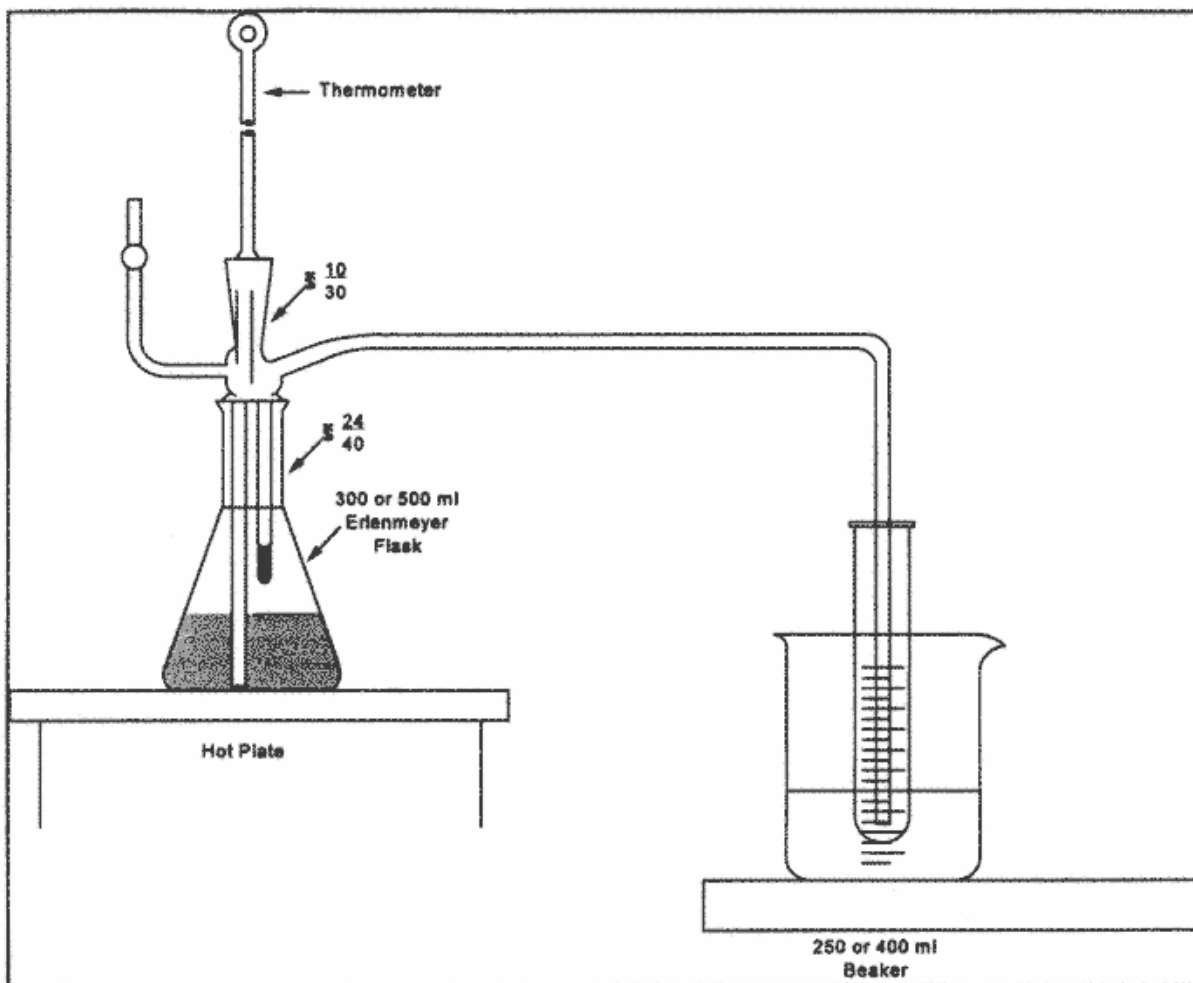
Figure 108C-1. Distillation Apparatus.
